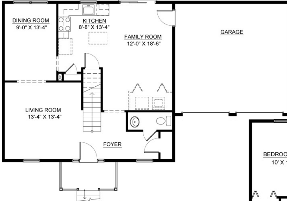
First Floor Plan B
